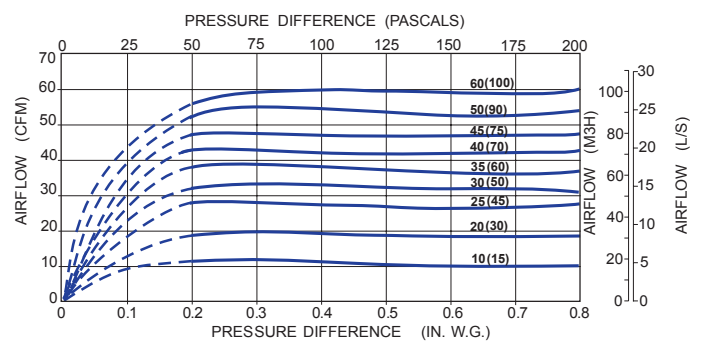
ZRT-1-4 or ZRT-2-4 – Maximum Flow Control ZRT-2-6 – Minimum Flow Control 4" Diameter Regulator (100 mm)
