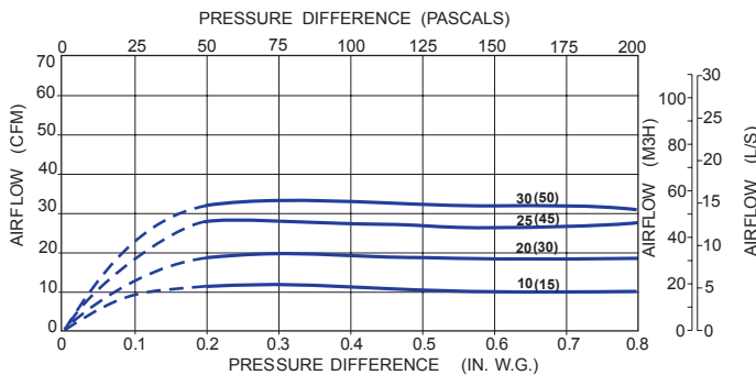
ZRT-1-6 or ZRT-2-6 – Maximum Flow Control 6" Diameter Regulator (150 mm)
