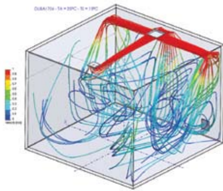
Bad installation with by-pass effect
